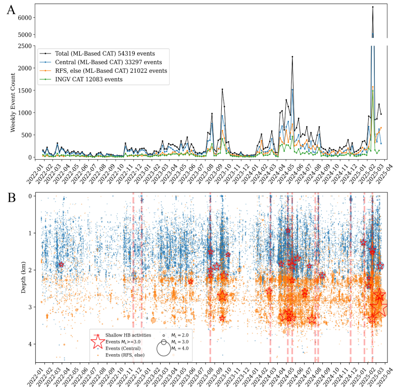
Fig. 2. Overview of the Campi Flegrei seismicity.
